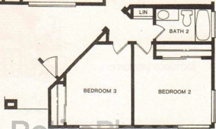
3 BEDROOM DESIGN
